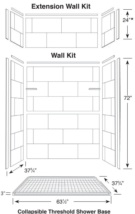
Shown with FC6338 Shower Base, X6382 Extension Wall Kit, GB3729PS Grab Bar Set, H2513 Shower Seat, GBHS18PS Hand Shower with 18" ADA grab bar.
